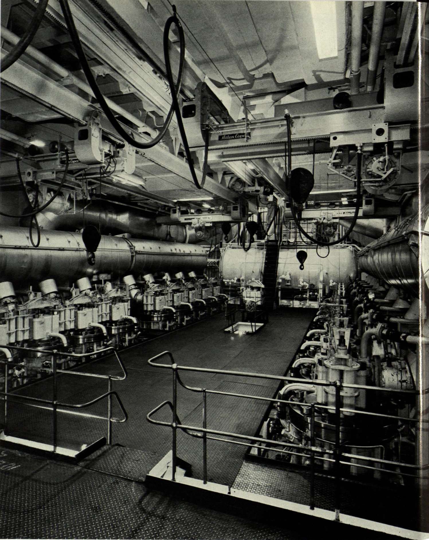
Five Atlas Copco compressed air cranes enable infinitely precise handling of main-engine parts in m/s Kungsholm, new 26,678 ton flagship of the Swedish American Line.
