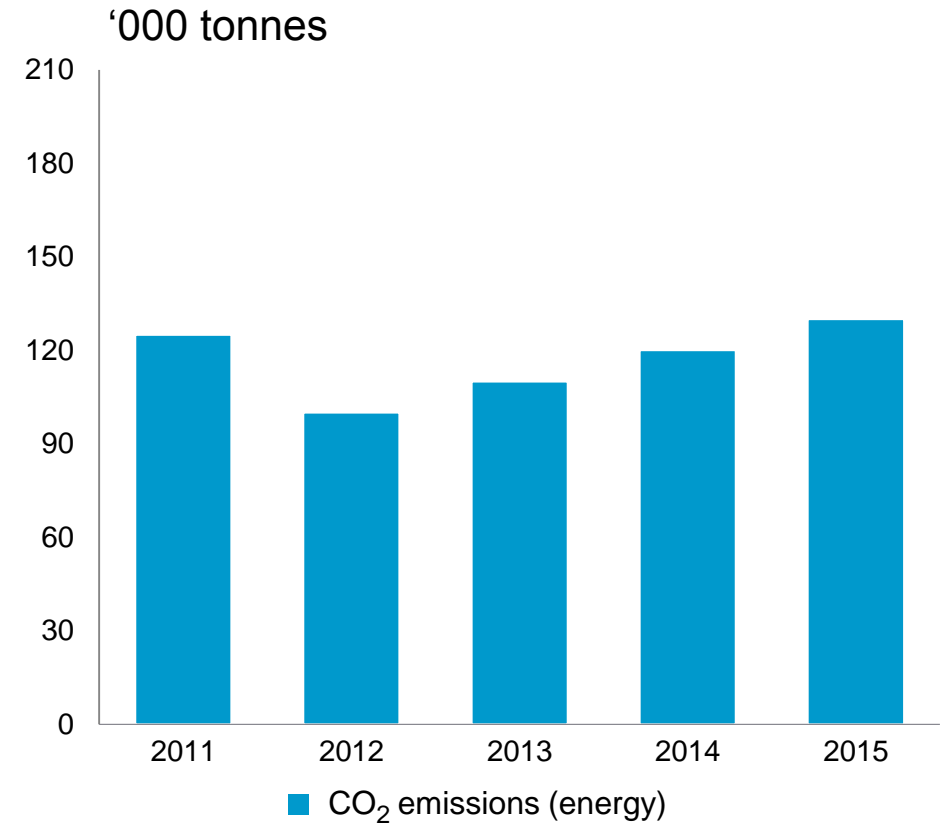
Co 2 emissions from energy
